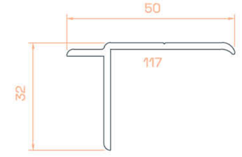
T - Kapama / T-Closure
