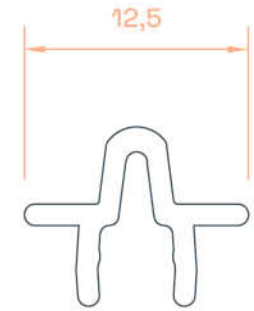
Sürme Ray / Sliding Rail
