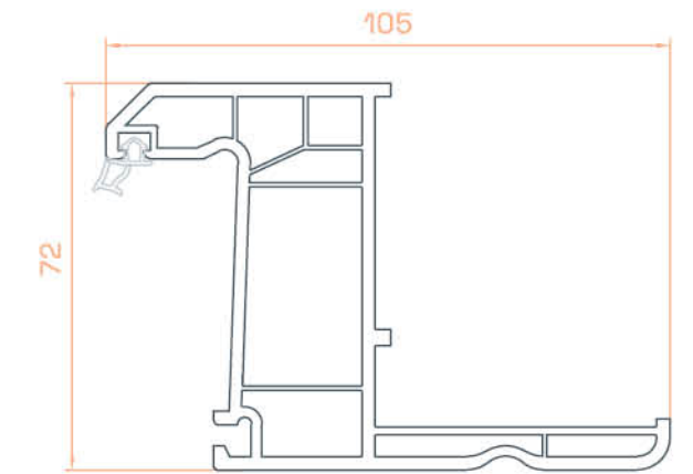
Pervazlı Kasa / Beaded Frame
