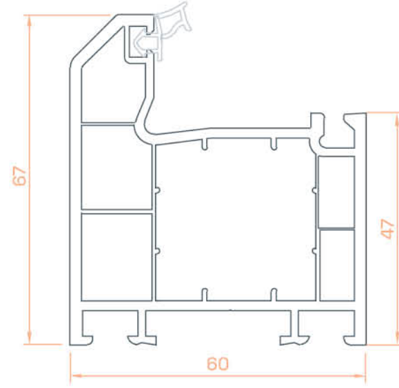
Kasa Profili / Case Profile
