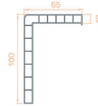
Pervaz / Trim / Casing
