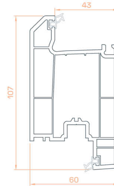
Kapı Kanat Profili / Door Wing Profile
