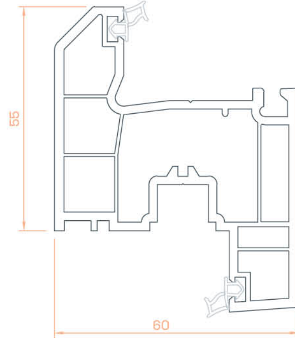
Kanat Profili / Wing Profile
