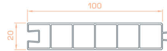
Lambiri / Paneling / Lath
