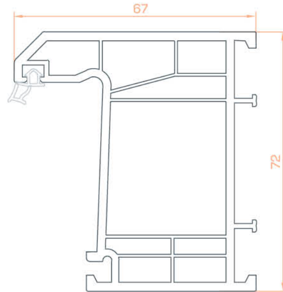
Kasa Profili / Case Profile
