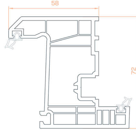
Kanat Profili / Wing Profile
